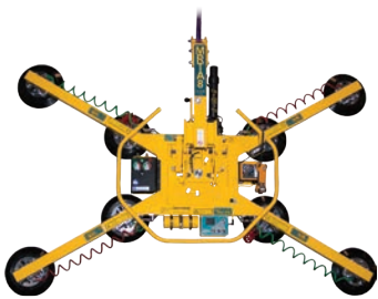
Quadra-Tilt™ Rotator 1400 (DC) w/ Intelli-Grip™ ..... MRTA811LDC3
